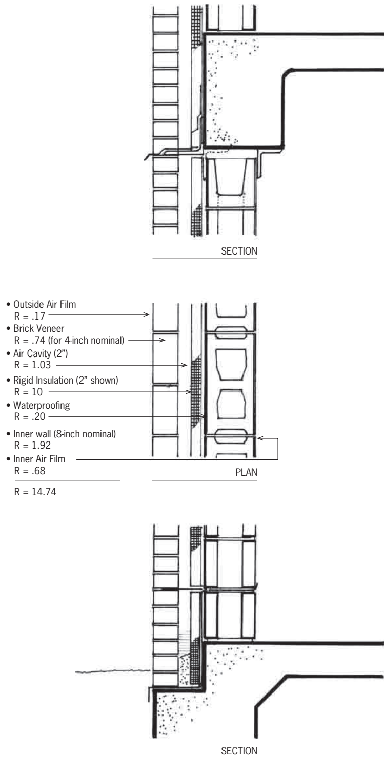
FIGURE 1.9 Overall thermal resistance (R-value) is defined by the composite of the enclosure component material R-values.
