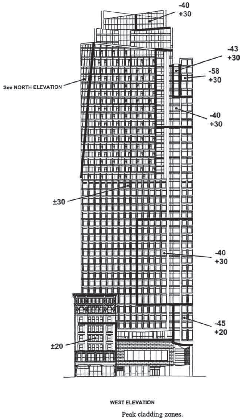
FIGURE 1.14b Building elevation with wind pressure contours converted to block pressure areas per elevation. CPP Wind Engineering
